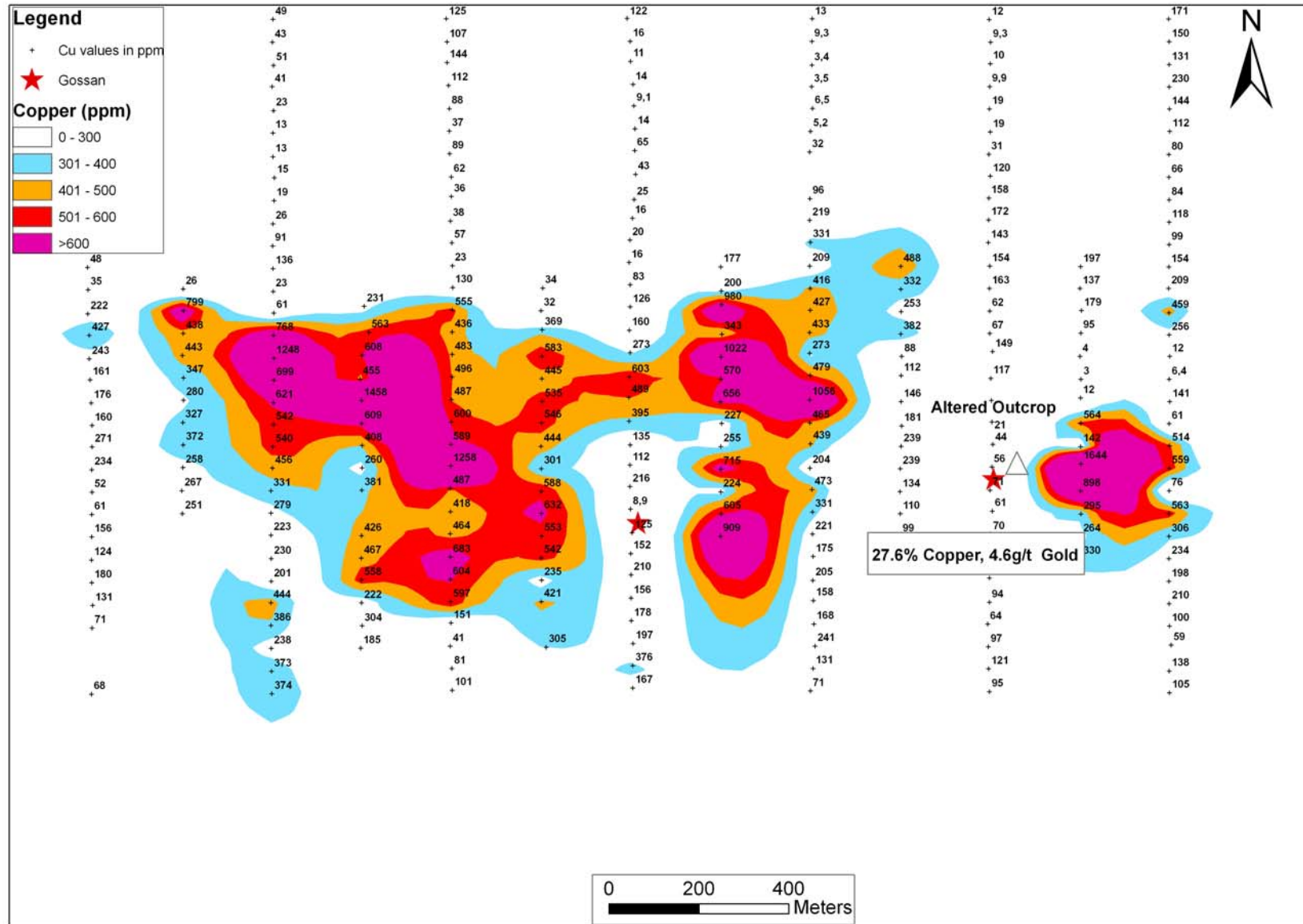
Figure 6: Copper (ppm) in Soil Anomaly at Prospect RN-11
