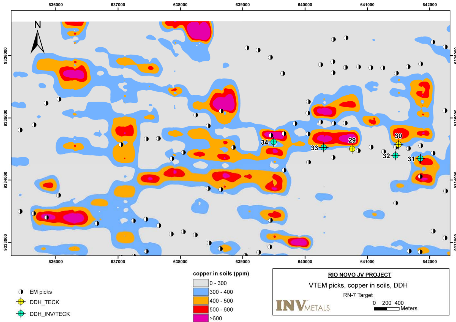
Figure 1: Copper in Soil Anomalies, VTEM Conductors and Drill Holes at Prospect RN-7
